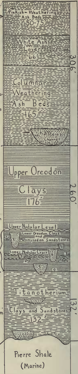
FIG. 1. Correlation diagram of sections of the White River formation. Section C: (1) algal ball horizon, Quinn Draw; (2) Metamynodon channel sandstone, Quinn Draw; (3), (4), (5) and (6) Metamynodon channel sandstones in Corral Draw; (7) Metamynodon channel sandstone, Little Corral Draw; (8) Solid sheet of algal limestone, Little Corral Draw; (9) Thin sheet of silicified limestone at base of Oreodon beds.
